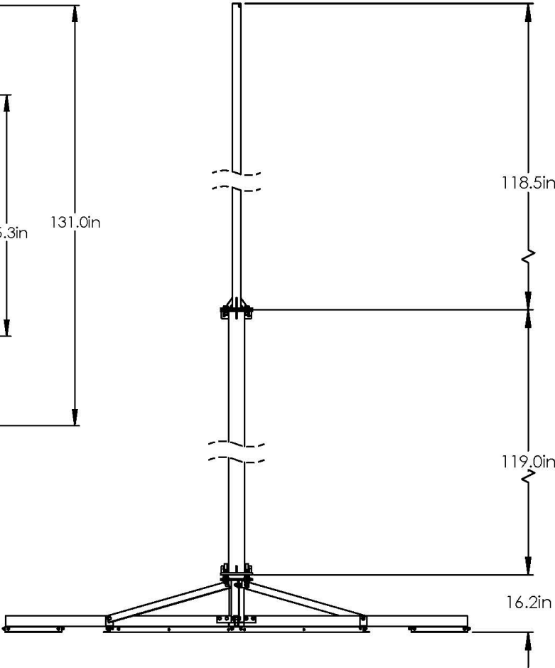
SIDE VIEW
